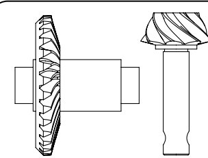
AX31530 AR44 Locker Bevel Gear Set 30T/8T x2
