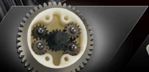
Planetary Differential
